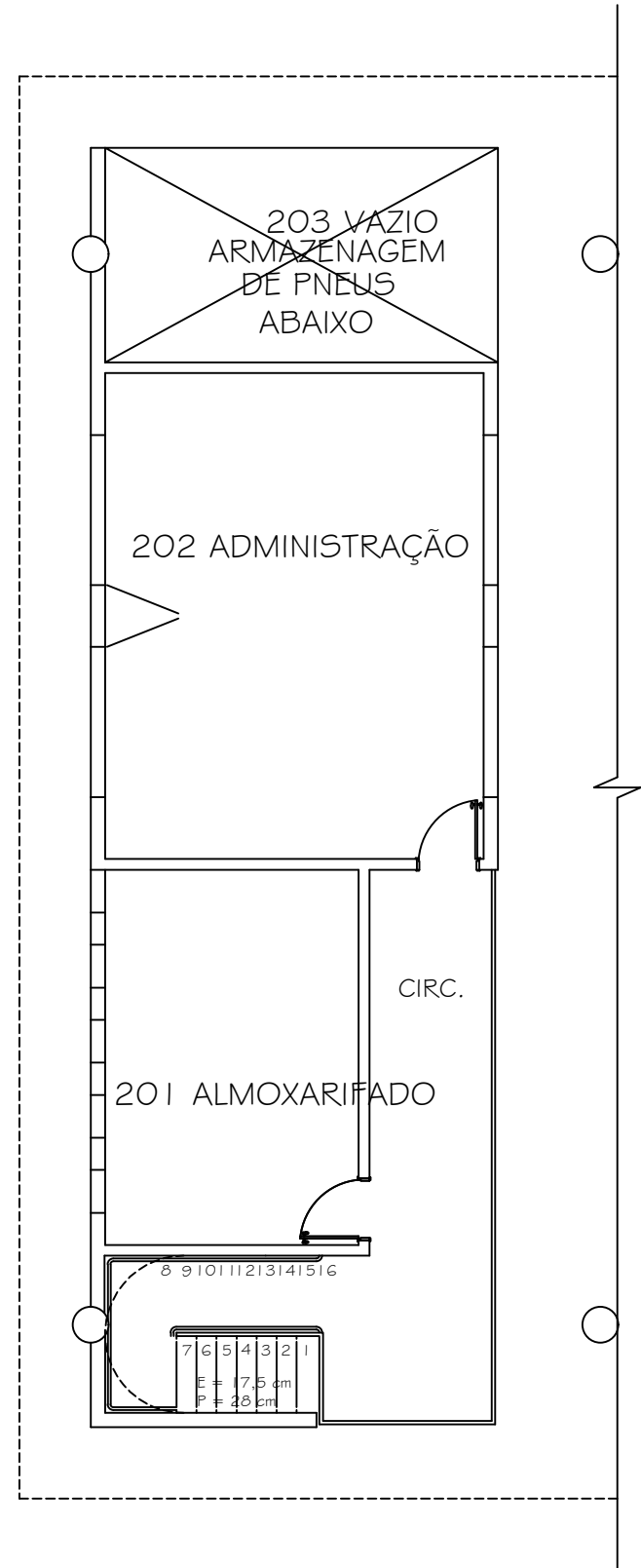
PLANTA LAYOUT MEZANINO
